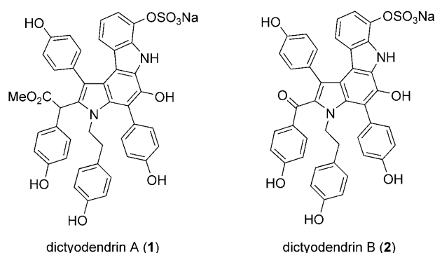
Scheme 1. Structures of dictyodendrin A ( 1 ) and B ( 2 ).
